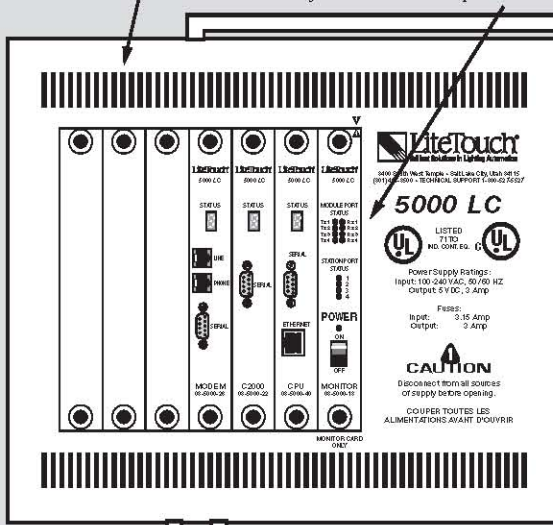
Front View (5000LC)
