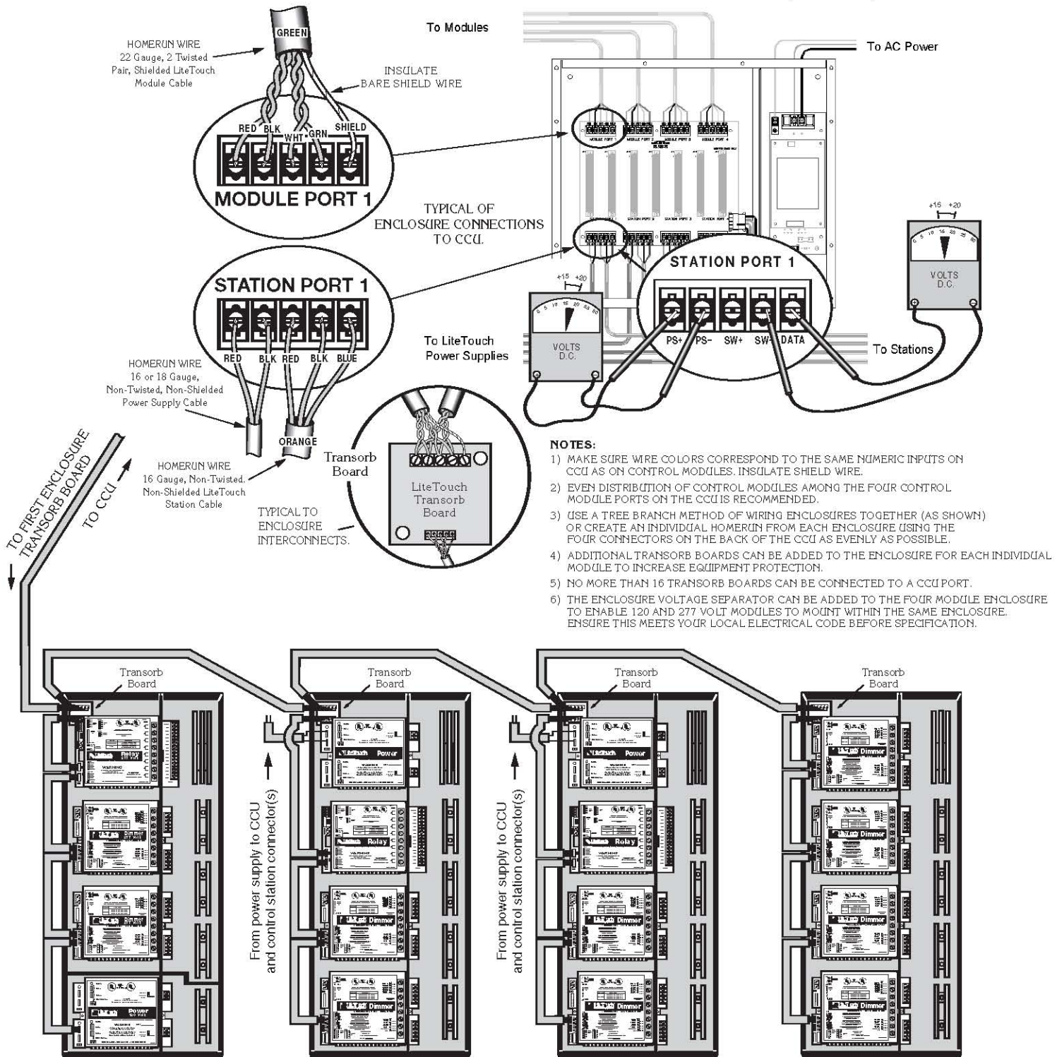
FRONT VIEW without lid (5000LC)
