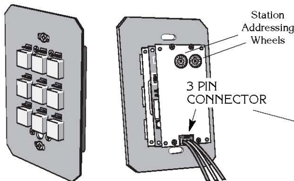
Front and Back Views of Control Station
